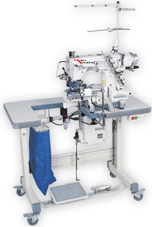
Direct Drive, High Speed, Cylinder-Bed, Interlock Machine. (Attaching For Knit Elastic Waistband)(With right hand knife)(With rear puller) (Pneumatic Top / under Thread Trimming Device & Venturi Device)(3-needle, 5-thread) (With Special Coating).
